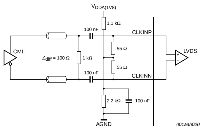
Fig 9. Interfacing CML to LVDS
